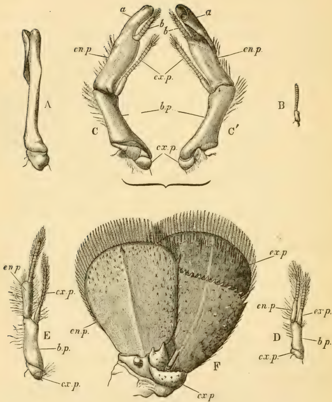
FIG 37.— Astacus fluviatilis .—Appendages of the left side of the abdomen ( \times 3 ). A, the posterior face of the first appendage of the male; B, the same of the female; C, posterior, and C', anterior faces of the second appendage of the male; D, the third appendage of the male; E, the same of the female; F, the sixth appendage. a , the rolled plate of the endopodite; b , the jointed extremity of the same; b.p. , basipodite; c.x.p. , coxopodite; en.p. , endopodite; ex.p. , exopodite.
